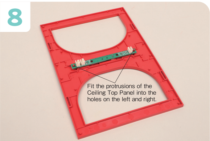
To assemble the Circuit Board, fit the protrusions of the Ceiling Top Panel into the holes on the left and right.
