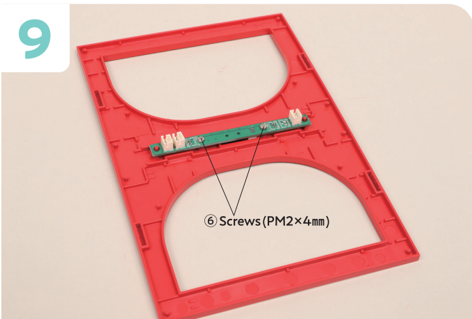
Tighten a ⑥ Screw (PM2×4mm) into each hole on the left and right of the Circuit Board.
